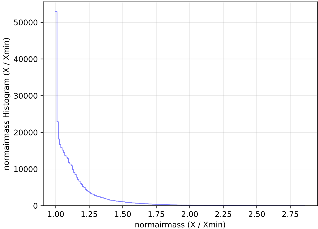
internal_u_expt27_nscale1.0v3.4_10yrs All sky y band: normairmass Histogram
