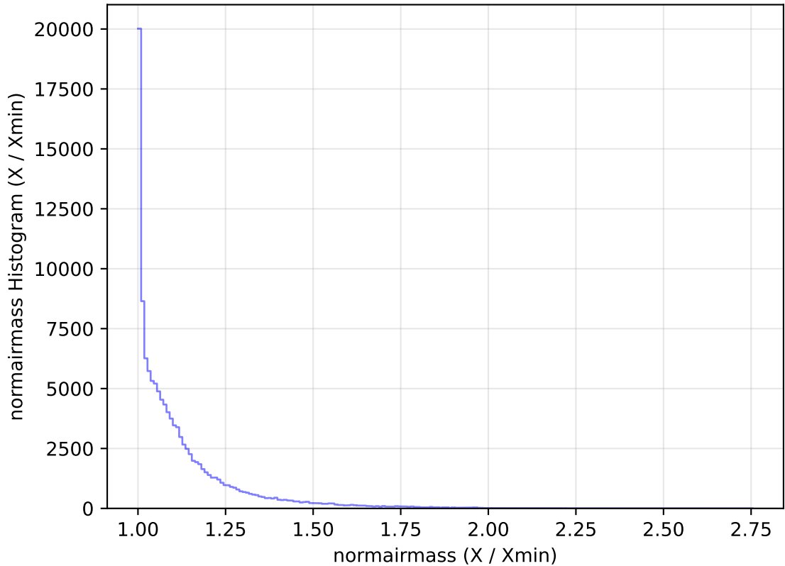
internal_u_expt27_nscale1.0v3.4_10yrs All sky u band: normairmass Histogram
