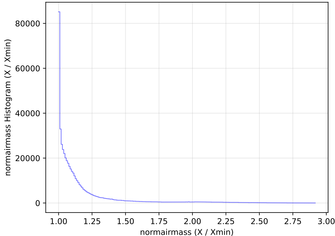
internal_u_expt27_nscale1.0v3.4_10yrs All sky i band: normairmass Histogram
