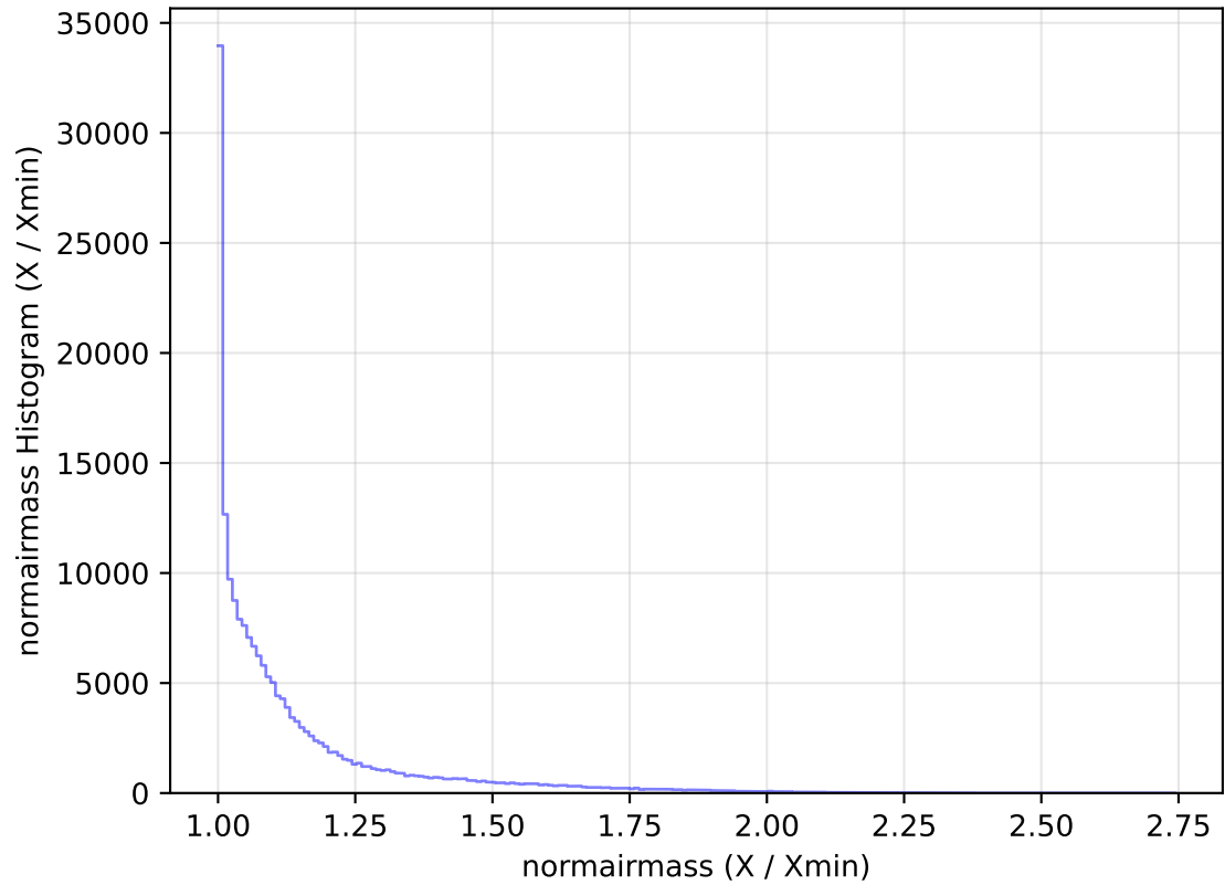
internal_u_expt27_nscale1.0v3.4_10yrs All sky g band: normairmass Histogram
