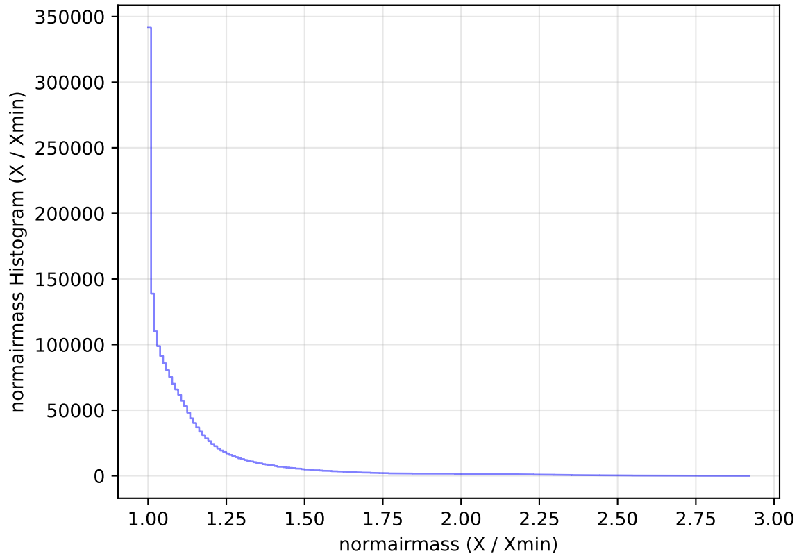
internal_u_expt27_nscale1.0v3.4_10yrs All sky all bands: normairmass Histogram
