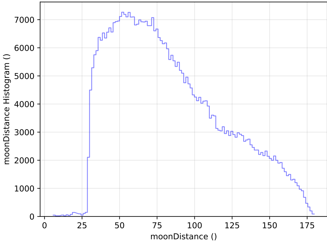
internal_u_expt27_nscale1.0v3.4_10yrs WFD z band: moonDistance Histogram
