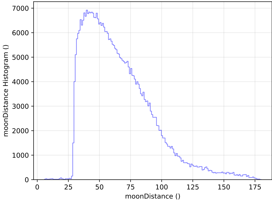
internal_u_expt27_nscale1.0v3.4_10yrs WFD y band: moonDistance Histogram
