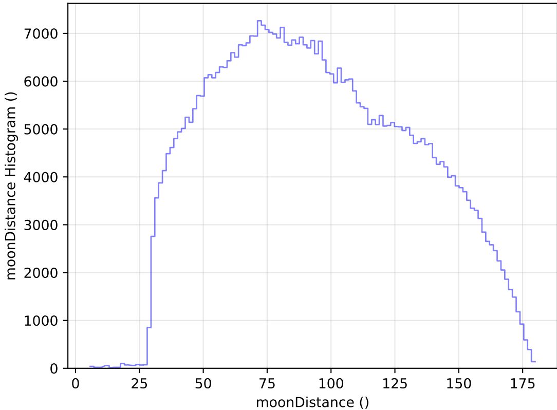
internal_u_expt27_nscale1.0v3.4_10yrs WFD i band: moonDistance Histogram
