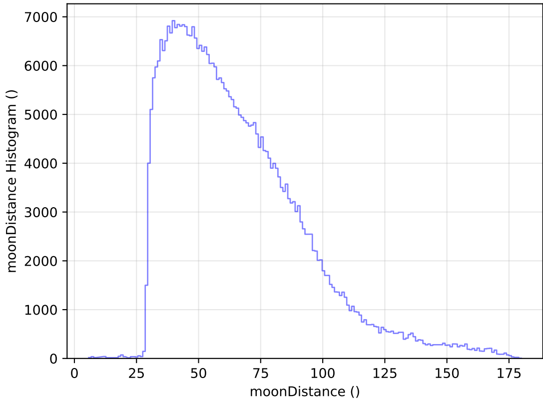
internal_u_expt27_nscale1.0v3.4_10yrs All sky y band: moonDistance Histogram
