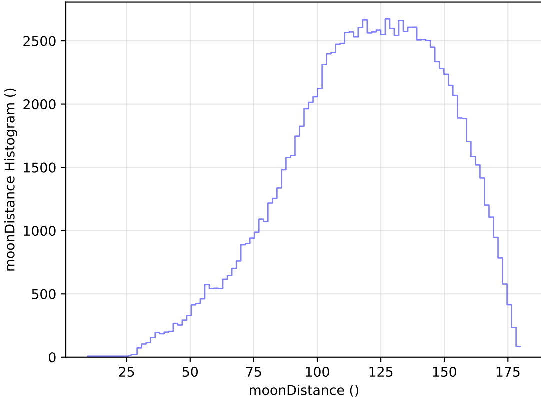
internal_u_expt27_nscale1.0v3.4_10yrs All sky u band: moonDistance Histogram
