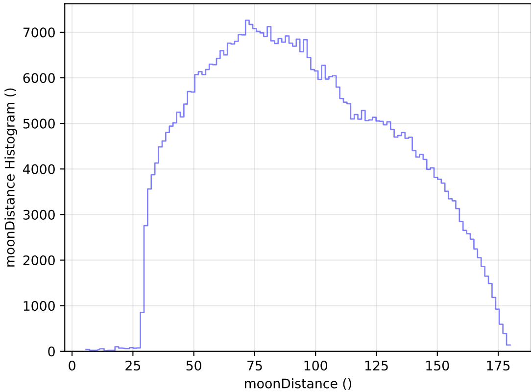
internal_u_expt27_nscale1.0v3.4_10yrs All sky i band: moonDistance Histogram
