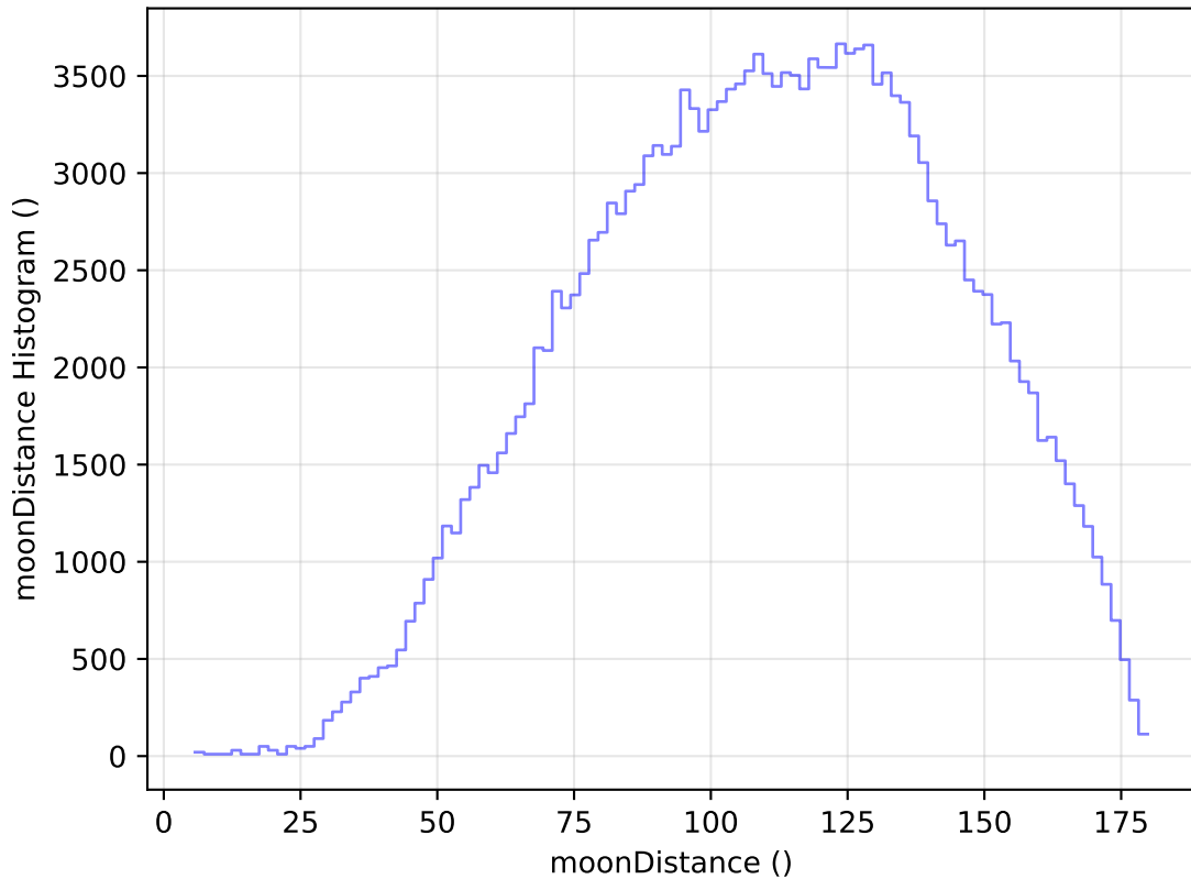
internal_u_expt27_nscale1.0v3.4_10yrs All sky g band: moonDistance Histogram
