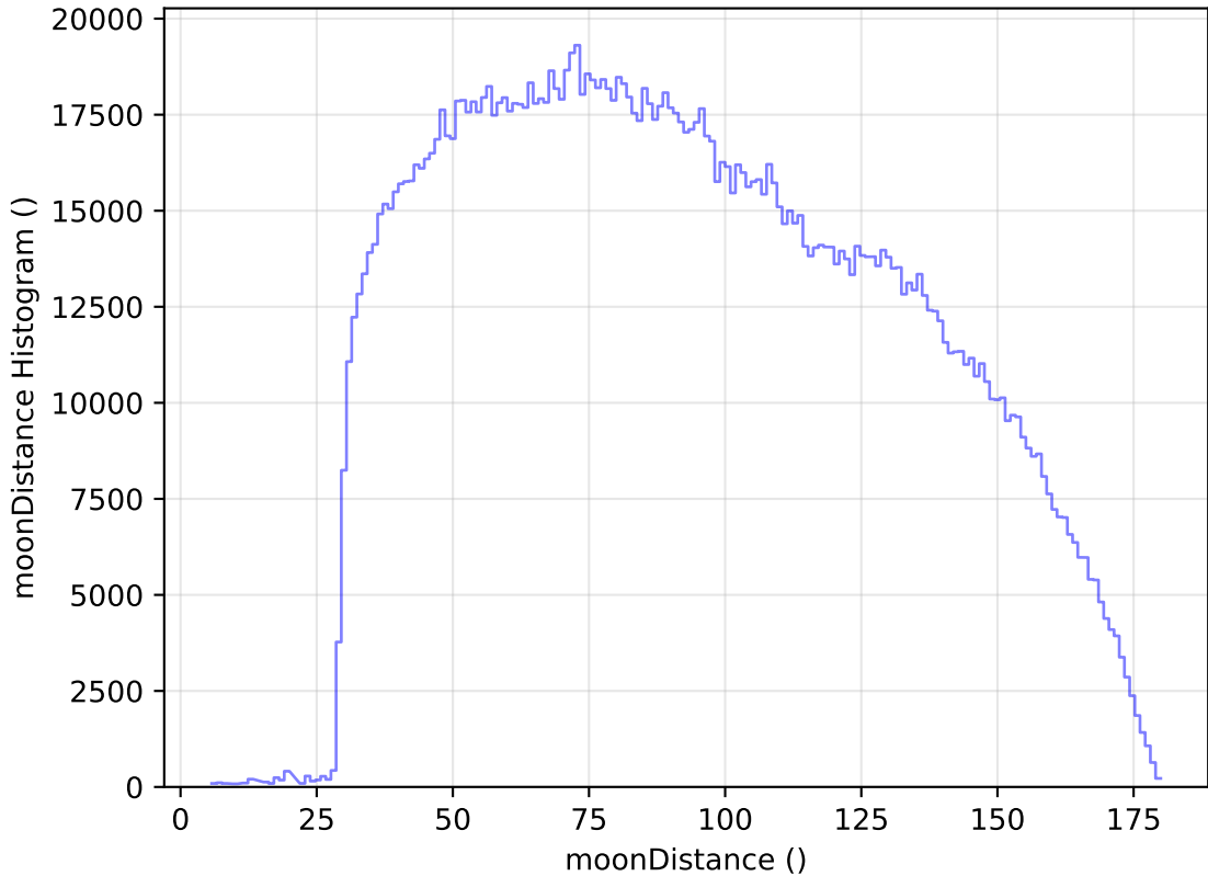
internal_u_expt27_nscale1.0v3.4_10yrs All sky all bands: moonDistance Histogram
