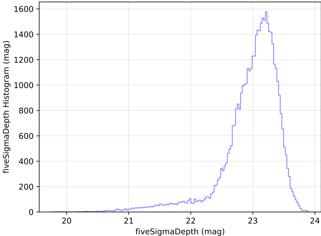
internal_u_expt27_nscale1.0v3.4_10yrs Yr 1 z band: fiveSigmaDepth Histogram
