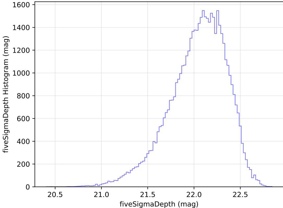
internal_u_expt27_nscale1.0v3.4_10yrs Yr 1 y band: fiveSigmaDepth Histogram
