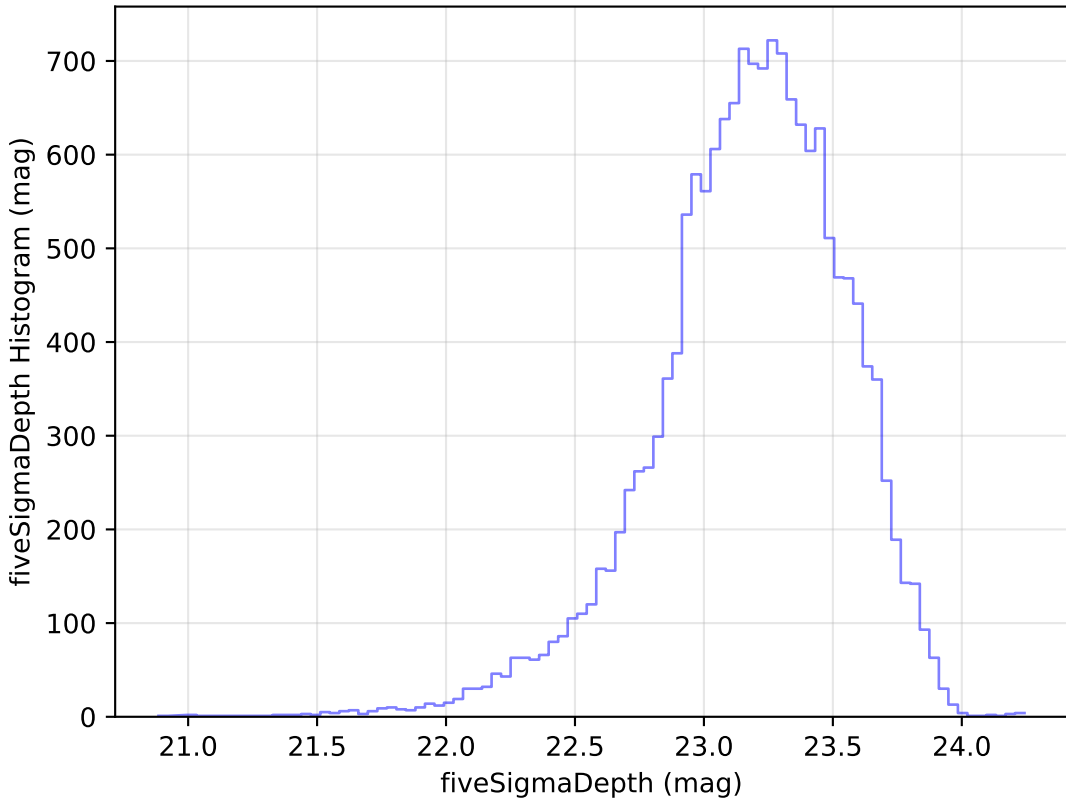
internal_u_expt27_nscale1.0v3.4_10yrs Yr 1 u band: fiveSigmaDepth Histogram
