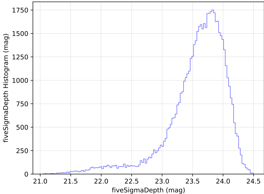
internal_u_expt27_nscale1.0v3.4_10yrs Yr 1 i band: fiveSigmaDepth Histogram
