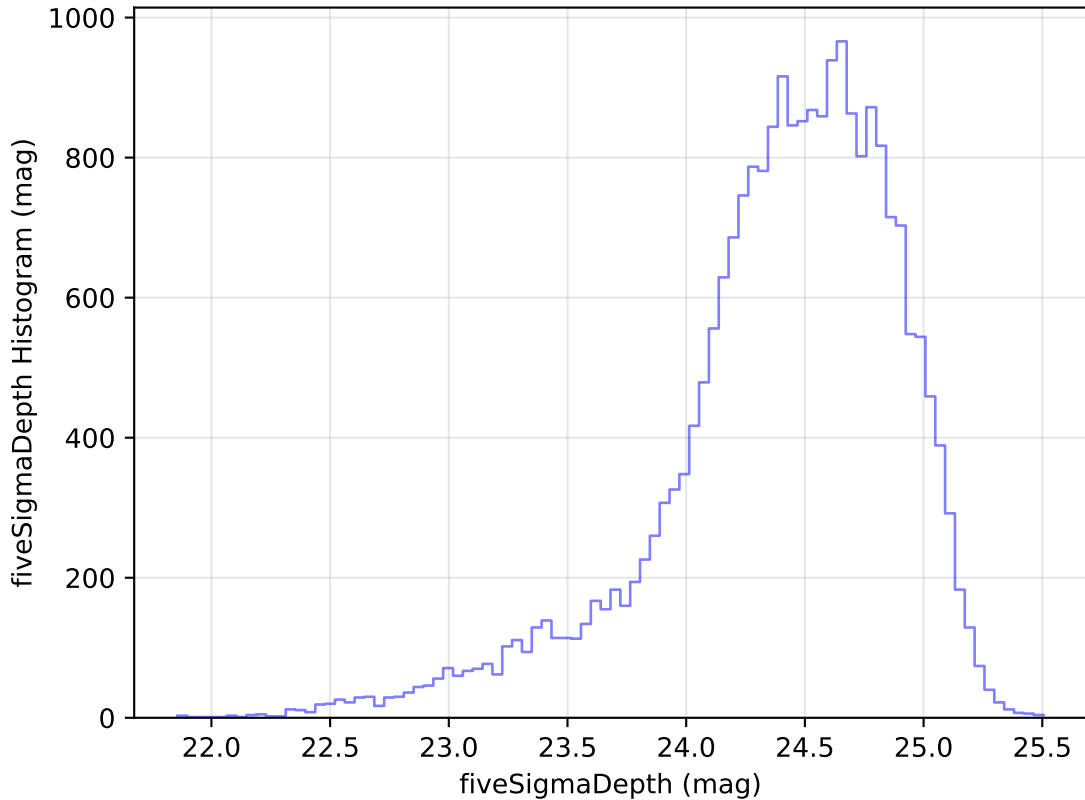
internal_u_expt27_nscale1.0v3.4_10yrs Yr 1 g band: fiveSigmaDepth Histogram
