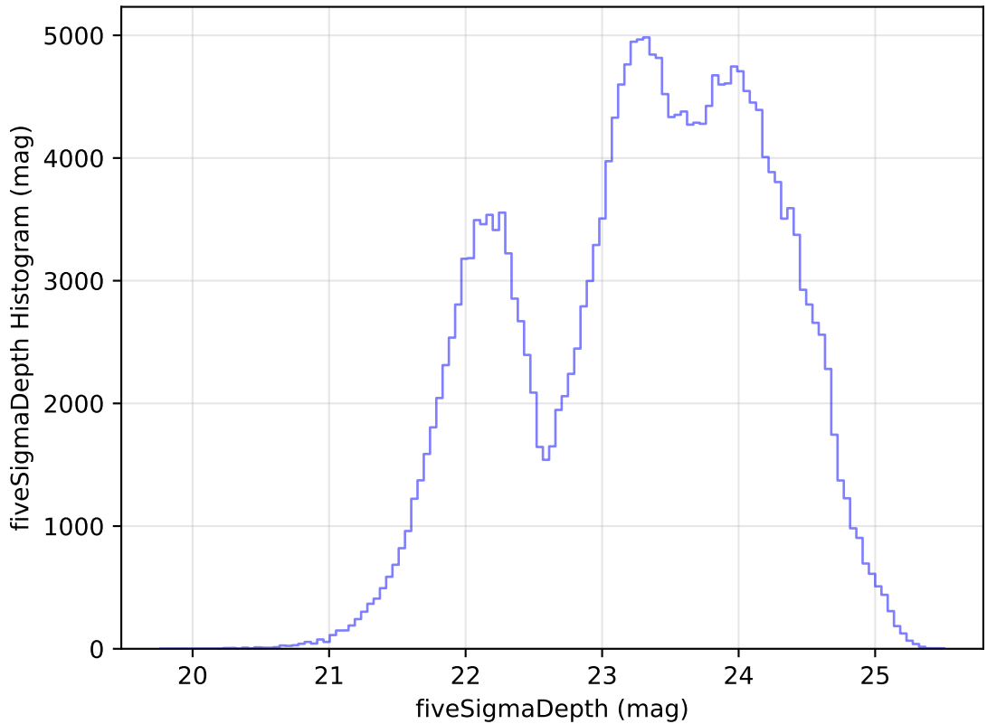
internal_u_expt27_nscale1.0v3.4_10yrs Yr 1 all bands: fiveSigmaDepth Histogram
