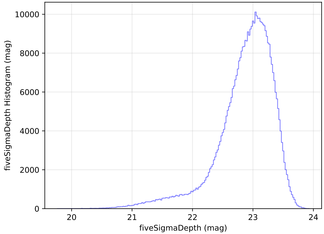
internal_u_expt27_nscale1.0v3.4_10yrs WFD z band: fiveSigmaDepth Histogram
