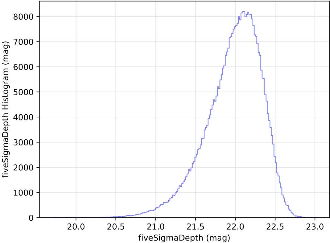
internal_u_expt27_nscale1.0v3.4_10yrs WFD y band: fiveSigmaDepth Histogram
