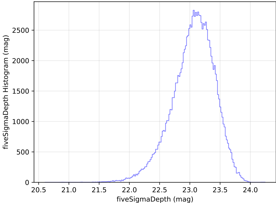
internal_u_expt27_nscale1.0v3.4_10yrs WFD u band: fiveSigmaDepth Histogram
