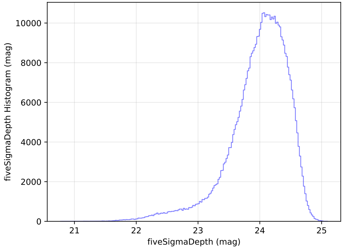
internal_u_expt27_nscale1.0v3.4_10yrs WFD r band: fiveSigmaDepth Histogram
