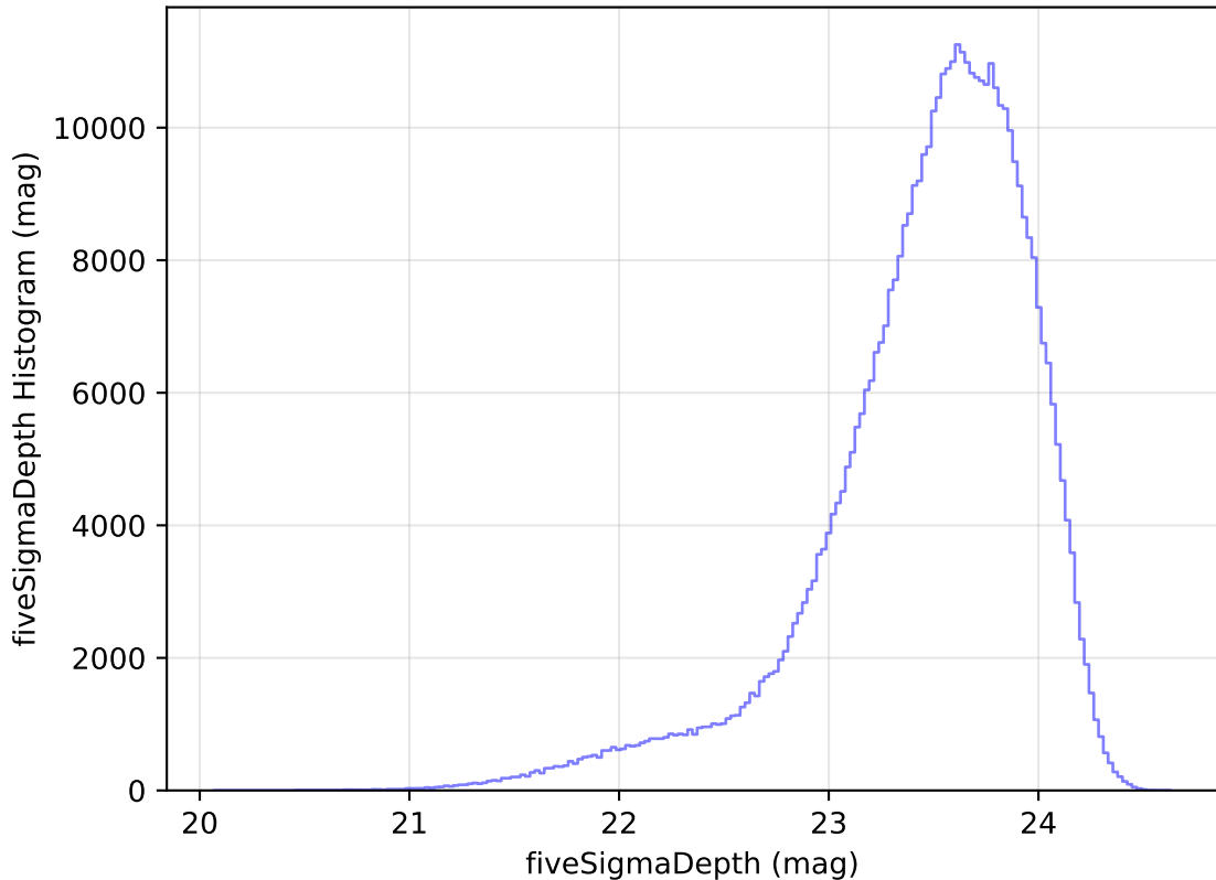
internal_u_expt27_nscale1.0v3.4_10yrs WFD i band: fiveSigmaDepth Histogram
