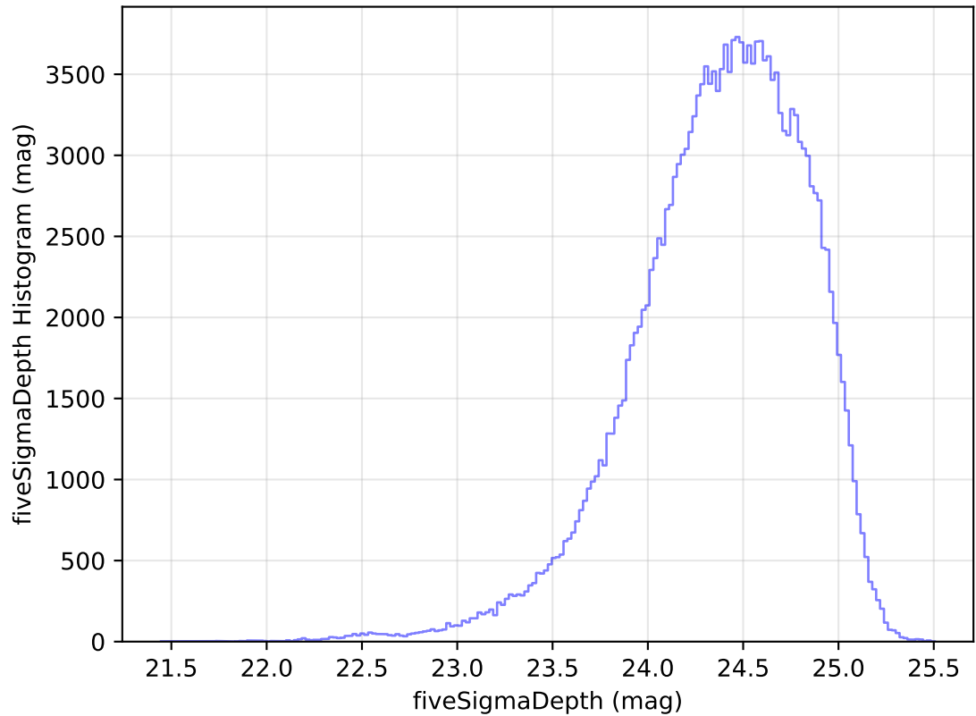
internal_u_expt27_nscale1.0v3.4_10yrs WFD g band: fiveSigmaDepth Histogram
