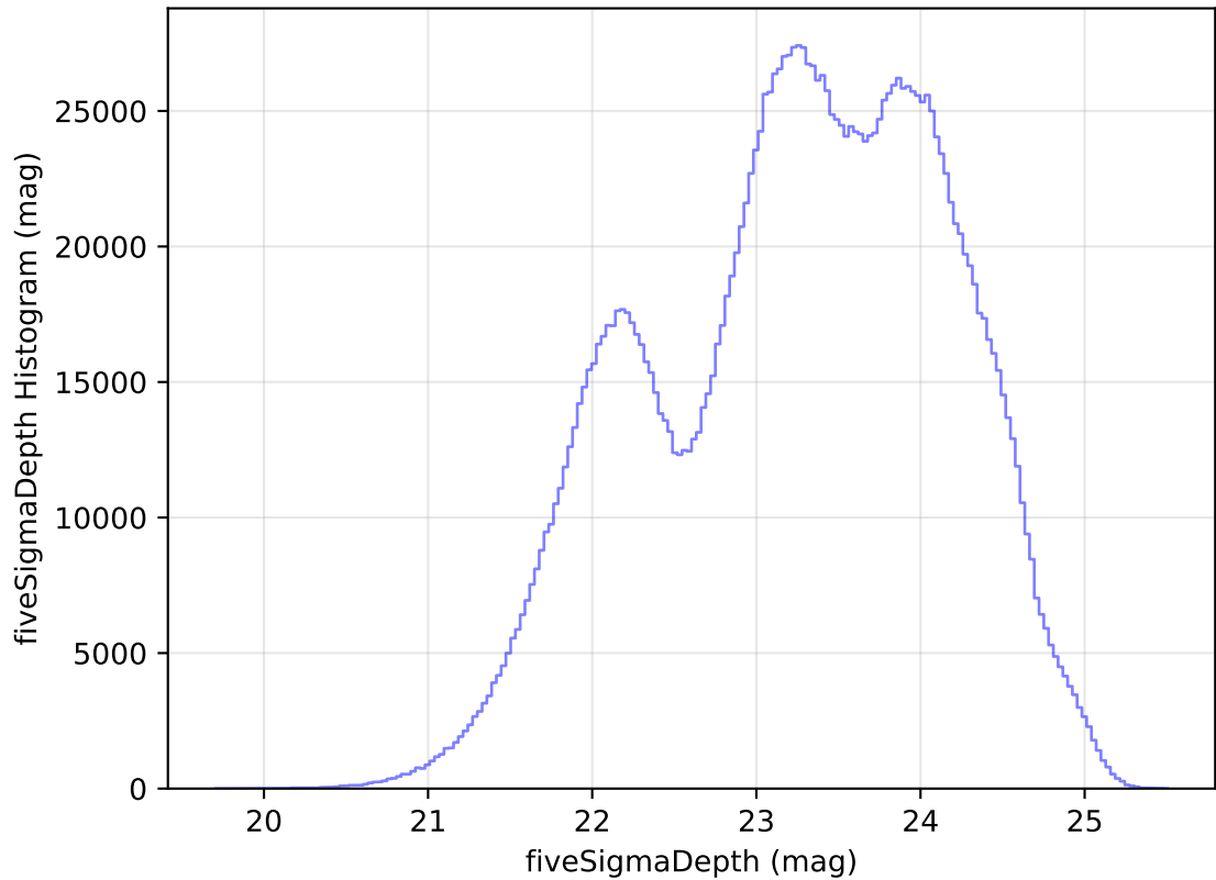
internal_u_expt27_nscale1.0v3.4_10yrs WFD all bands: fiveSigmaDepth Histogram
