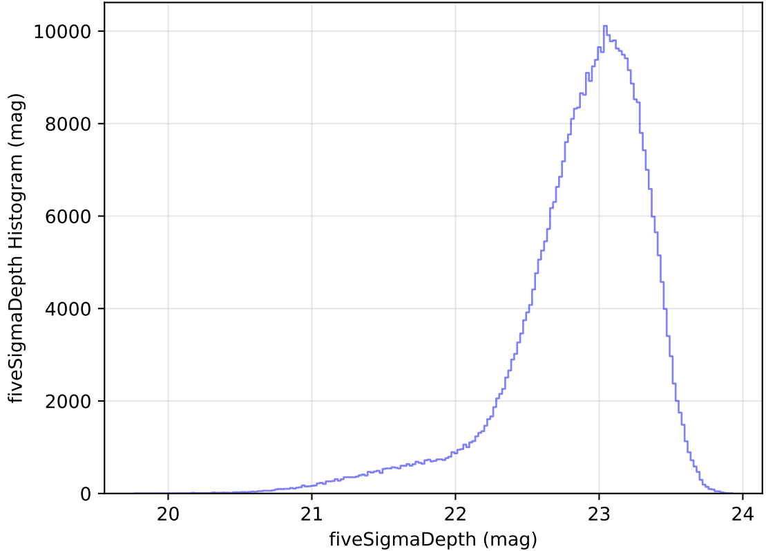
internal_u_expt27_nscale1.0v3.4_10yrs All sky z band: fiveSigmaDepth Histogram
