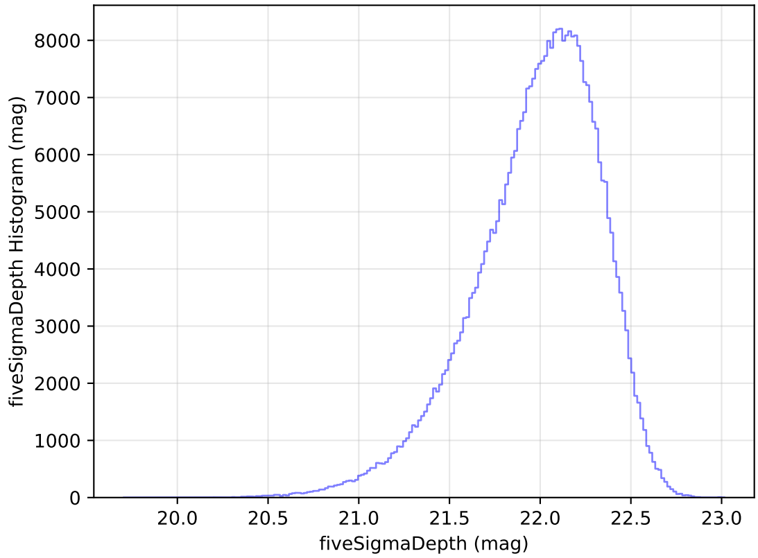
internal_u_expt27_nscale1.0v3.4_10yrs All sky y band: fiveSigmaDepth Histogram
