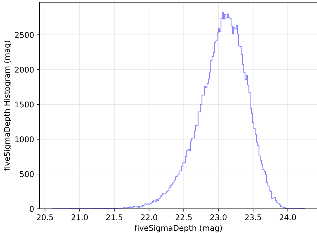
internal_u_expt27_nscale1.0v3.4_10yrs All sky u band: fiveSigmaDepth Histogram
