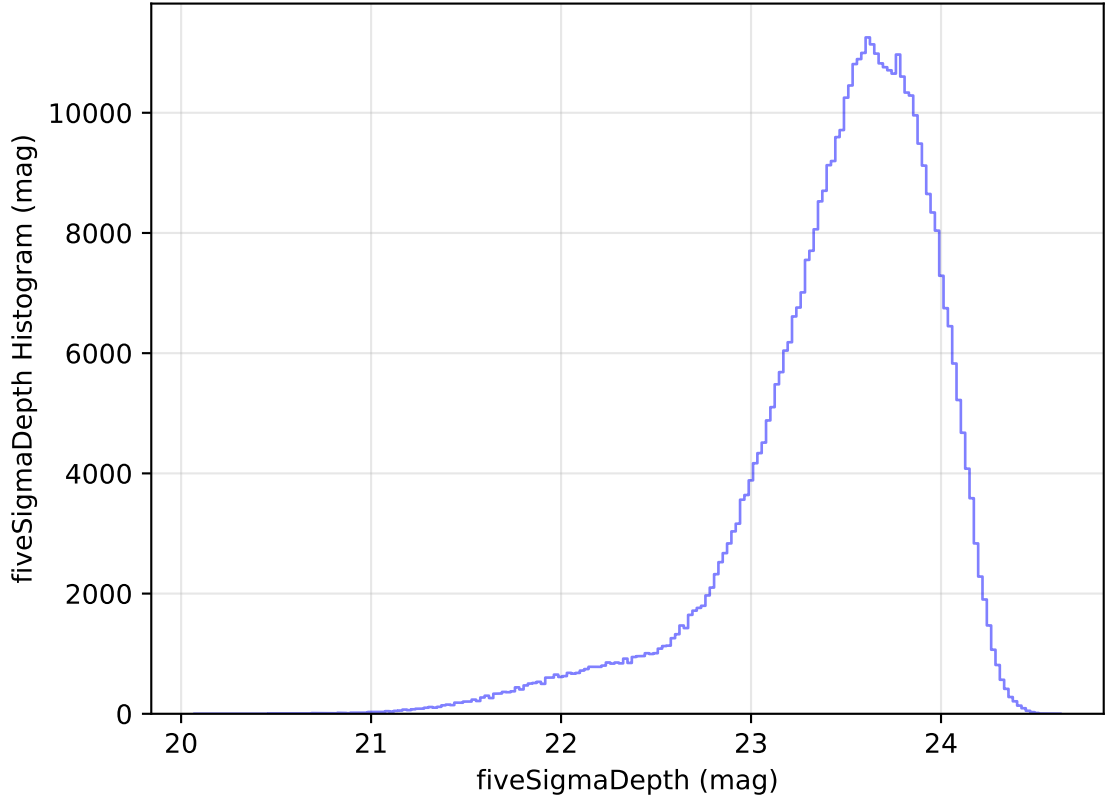
internal_u_expt27_nscale1.0v3.4_10yrs All sky i band: fiveSigmaDepth Histogram
