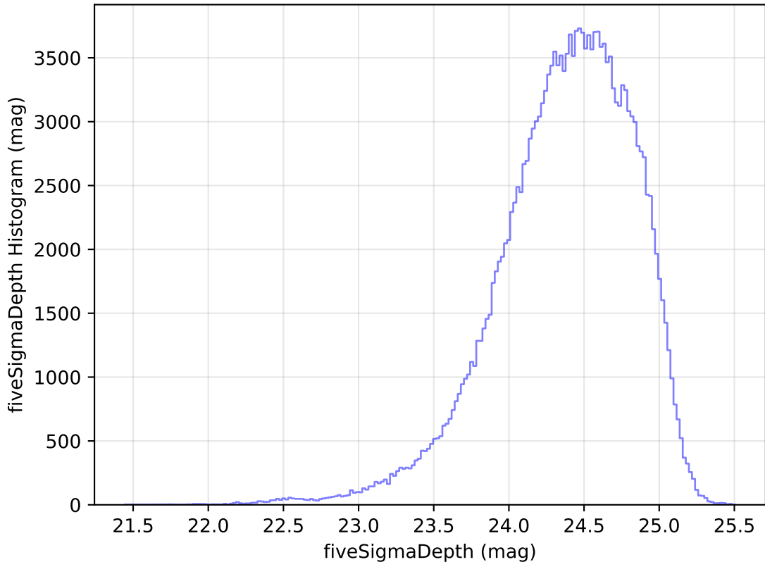
internal_u_expt27_nscale1.0v3.4_10yrs All sky g band: fiveSigmaDepth Histogram
