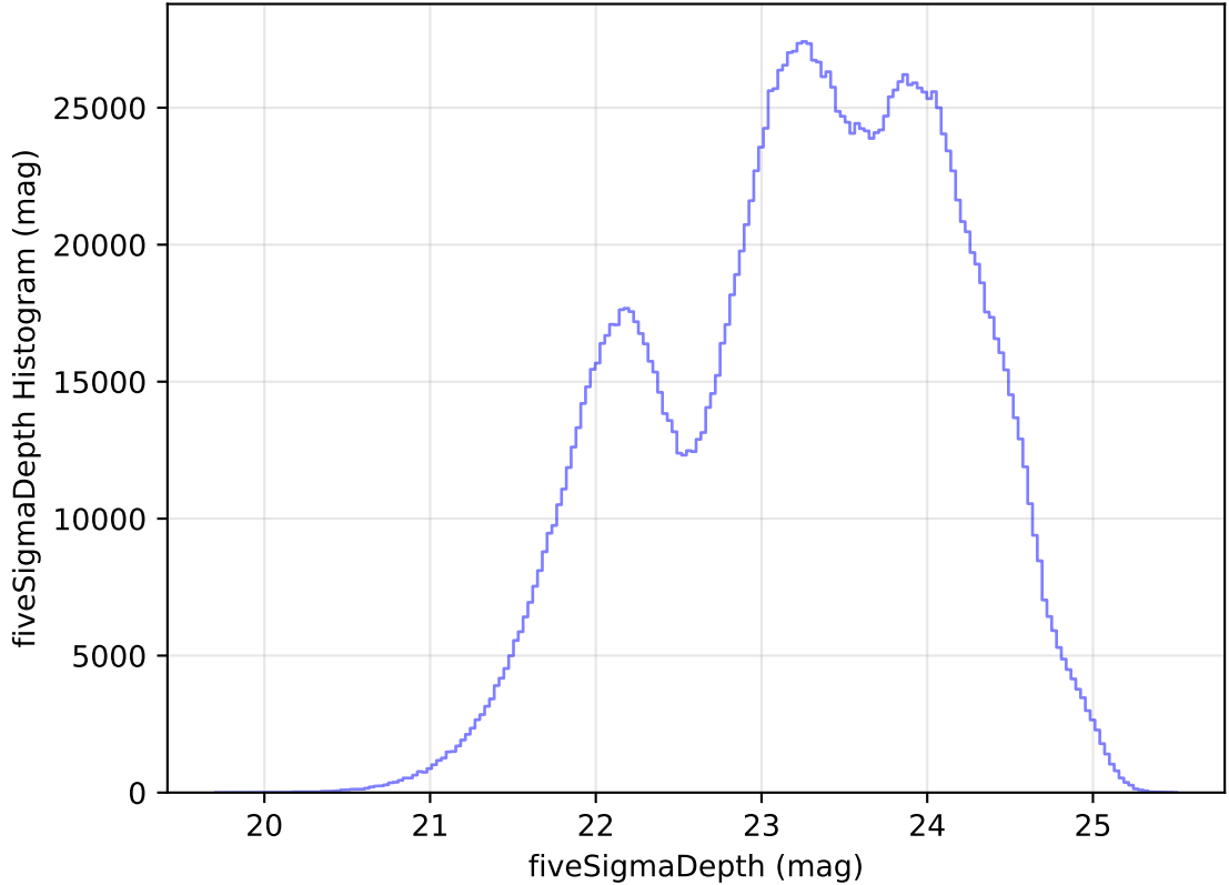
internal_u_expt27_nscale1.0v3.4_10yrs All sky all bands: fiveSigmaDepth Histogram
