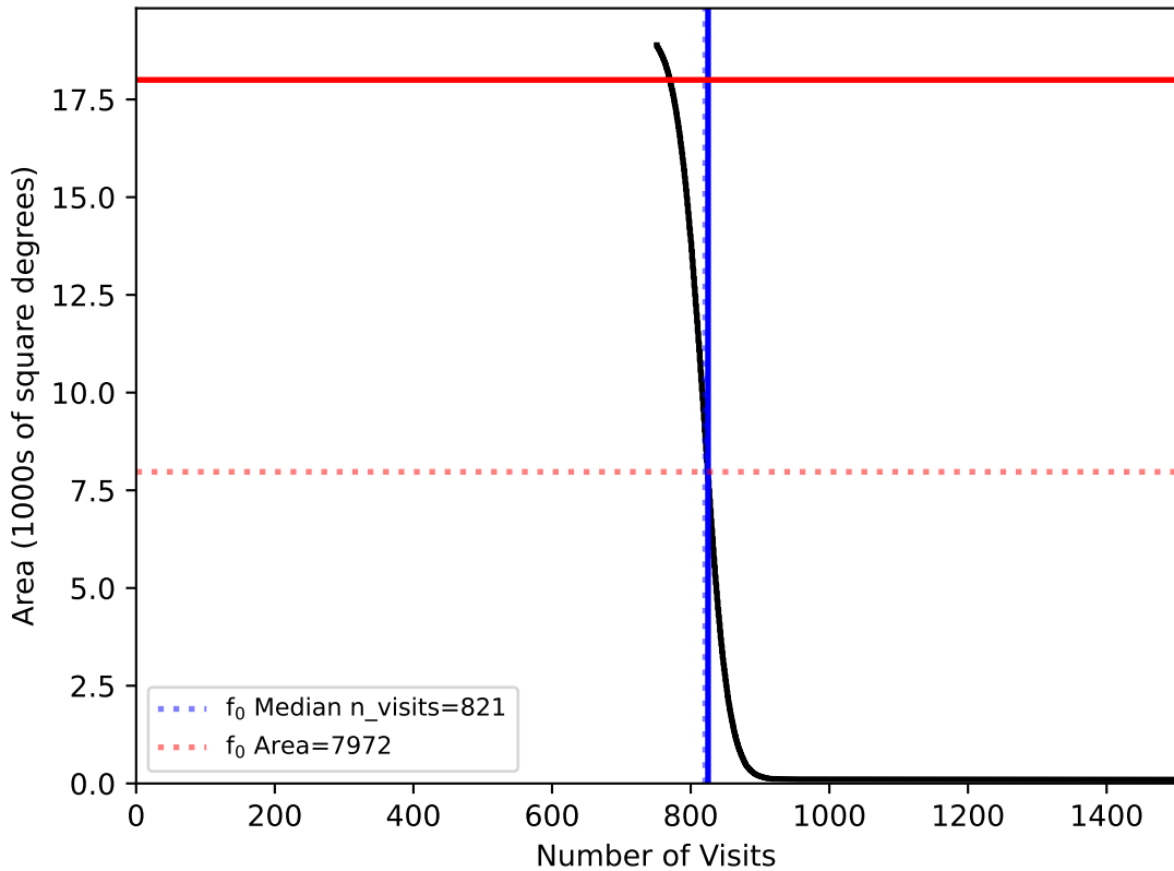
internal_u_expt27_nscale1.0v3.4_10yrs WFD: fO
