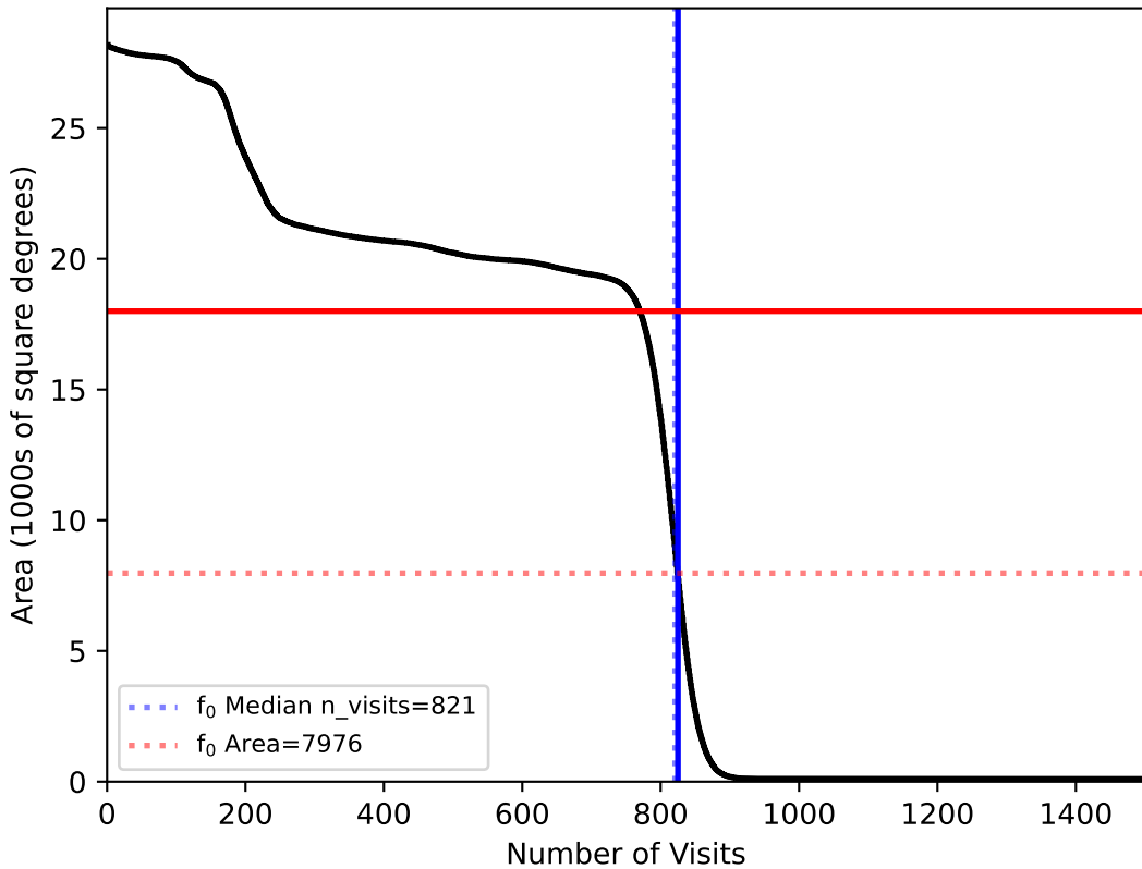
internal_u_expt27_nscale1.0v3.4_10yrs All sky: f0
