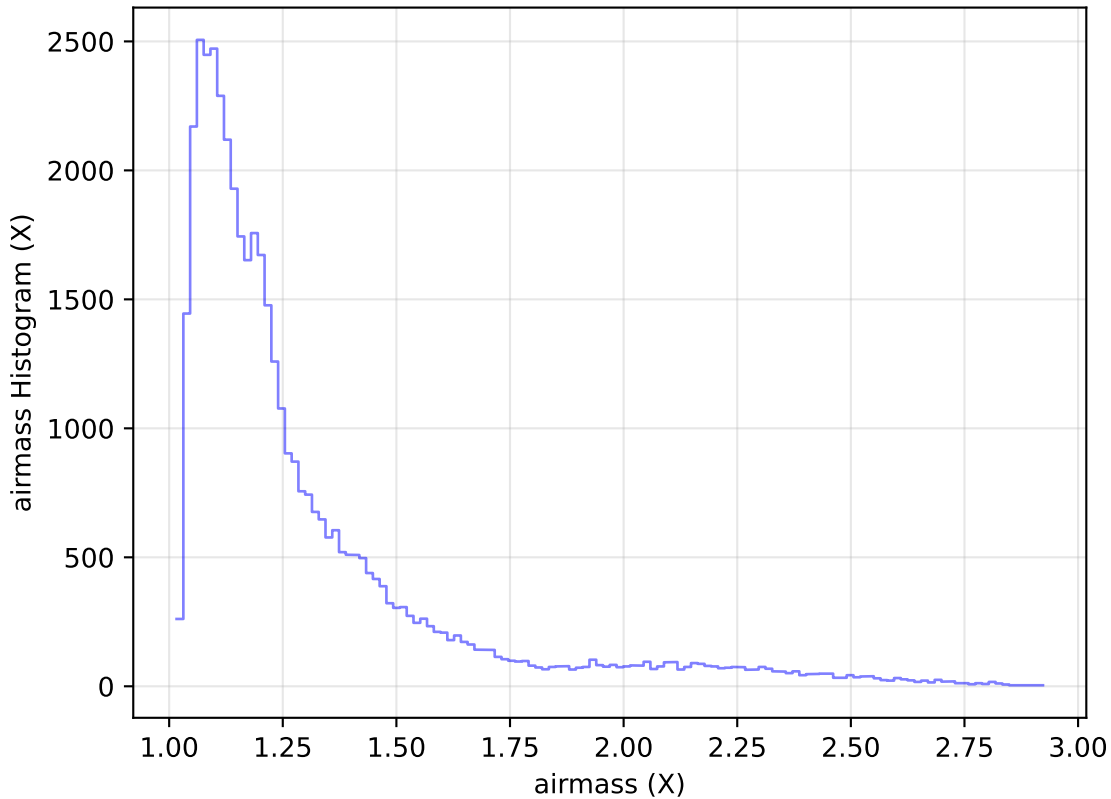
internal_u_expt27_nscale1.0v3.4_10yrs Yr 1 z band: airmass Histogram
