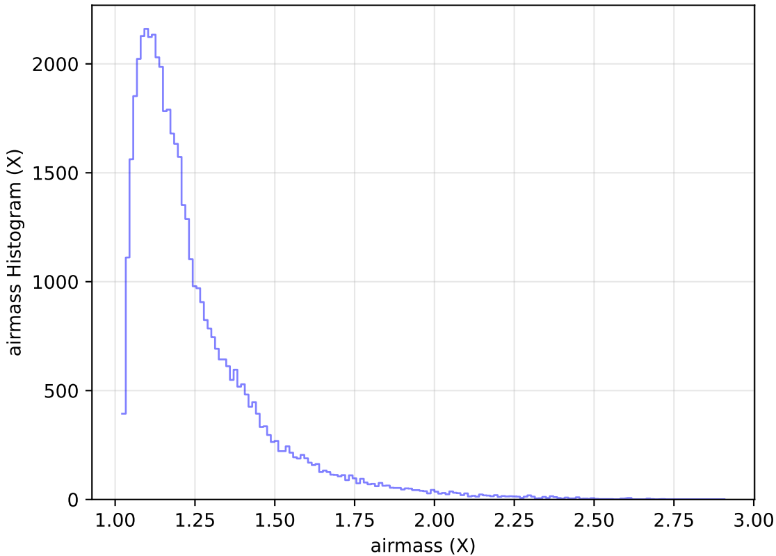
internal_u_expt27_nscale1.0v3.4_10yrs Yr 1 y band: airmass Histogram
