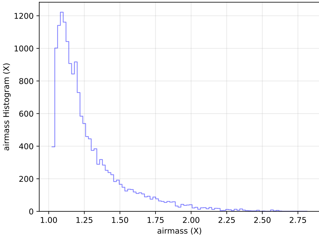
internal_u_expt27_nscale1.0v3.4_10yrs Yr 1 u band: airmass Histogram
