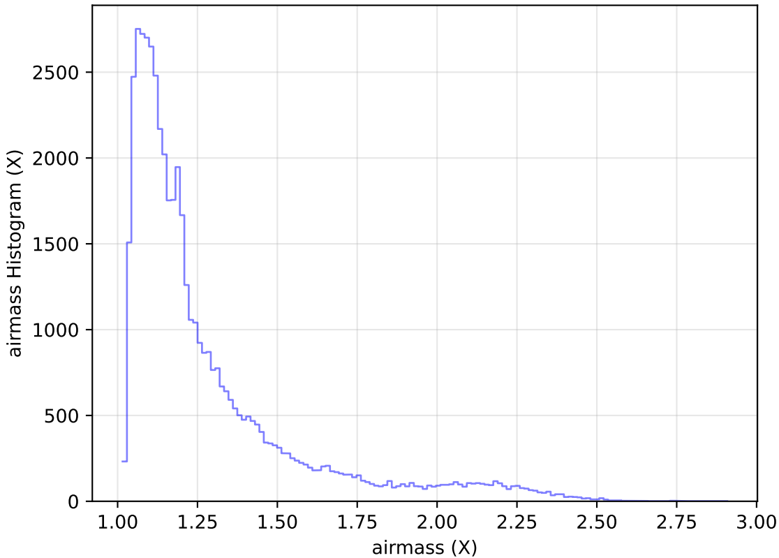
internal_u_expt27_nscale1.0v3.4_10yrs Yr 1 r band: airmass Histogram
