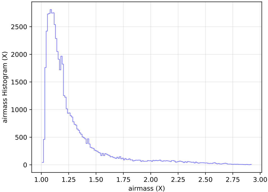
internal_u_expt27_nscale1.0v3.4_10yrs Yr 1 i band: airmass Histogram
