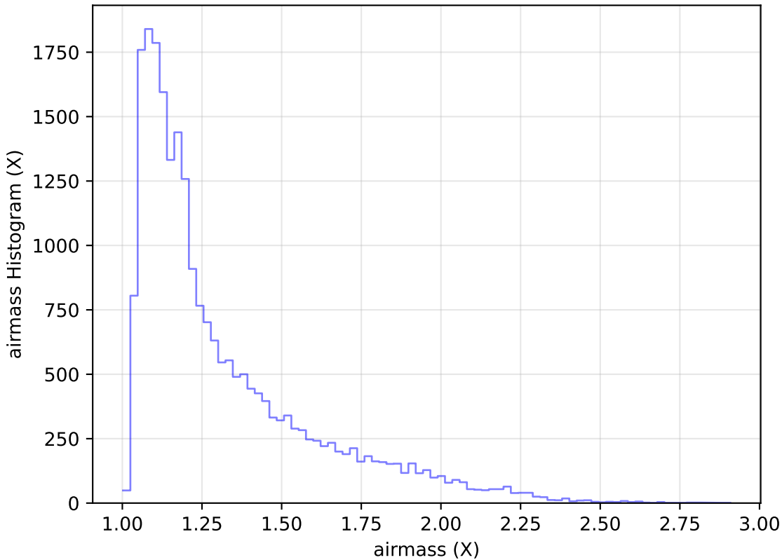
internal_u_expt27_nscale1.0v3.4_10yrs Yr 1 g band: airmass Histogram
