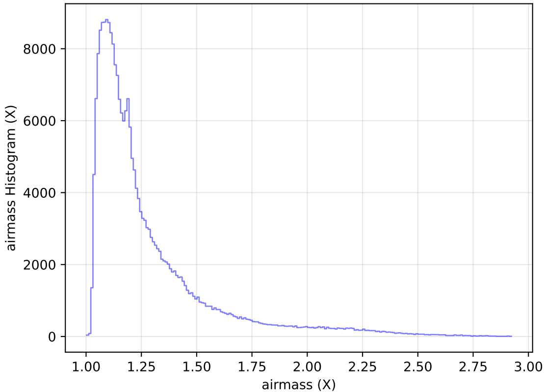
internal_u_expt27_nscale1.0v3.4_10yrs Yr 1 all bands: airmass Histogram
