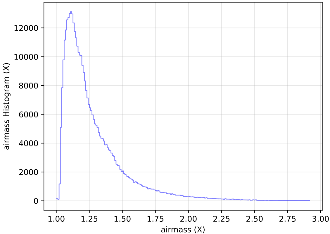
internal_u_expt27_nscale1.0v3.4_10yrs WFD y band: airmass Histogram
