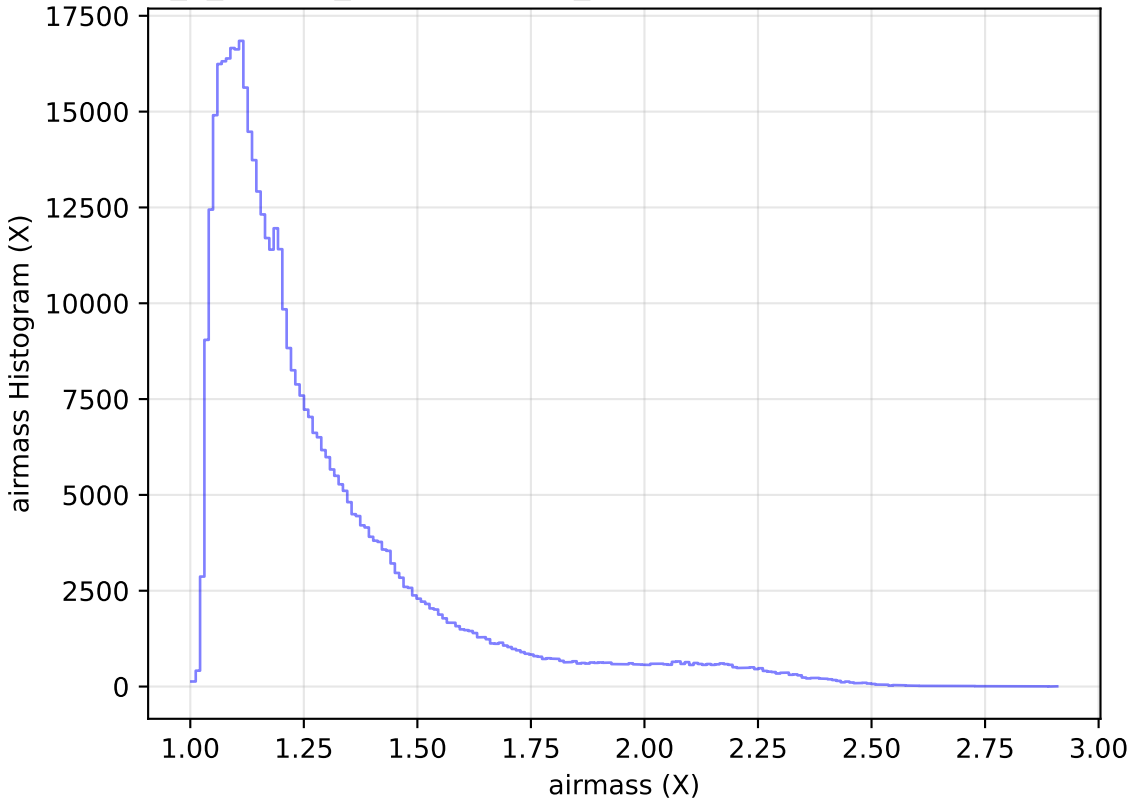
internal_u_expt27_nscale1.0v3.4_10yrs WFD r band: airmass Histogram
