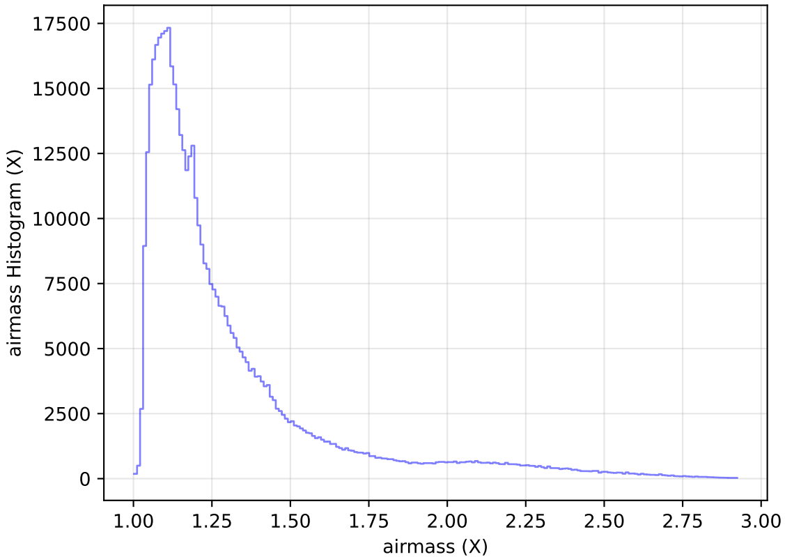
internal_u_expt27_nscale1.0v3.4_10yrs WFD i band: airmass Histogram
