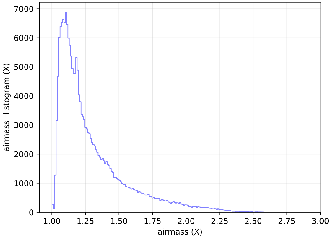
internal_u_expt27_nscale1.0v3.4_10yrs WFD g band: airmass Histogram
