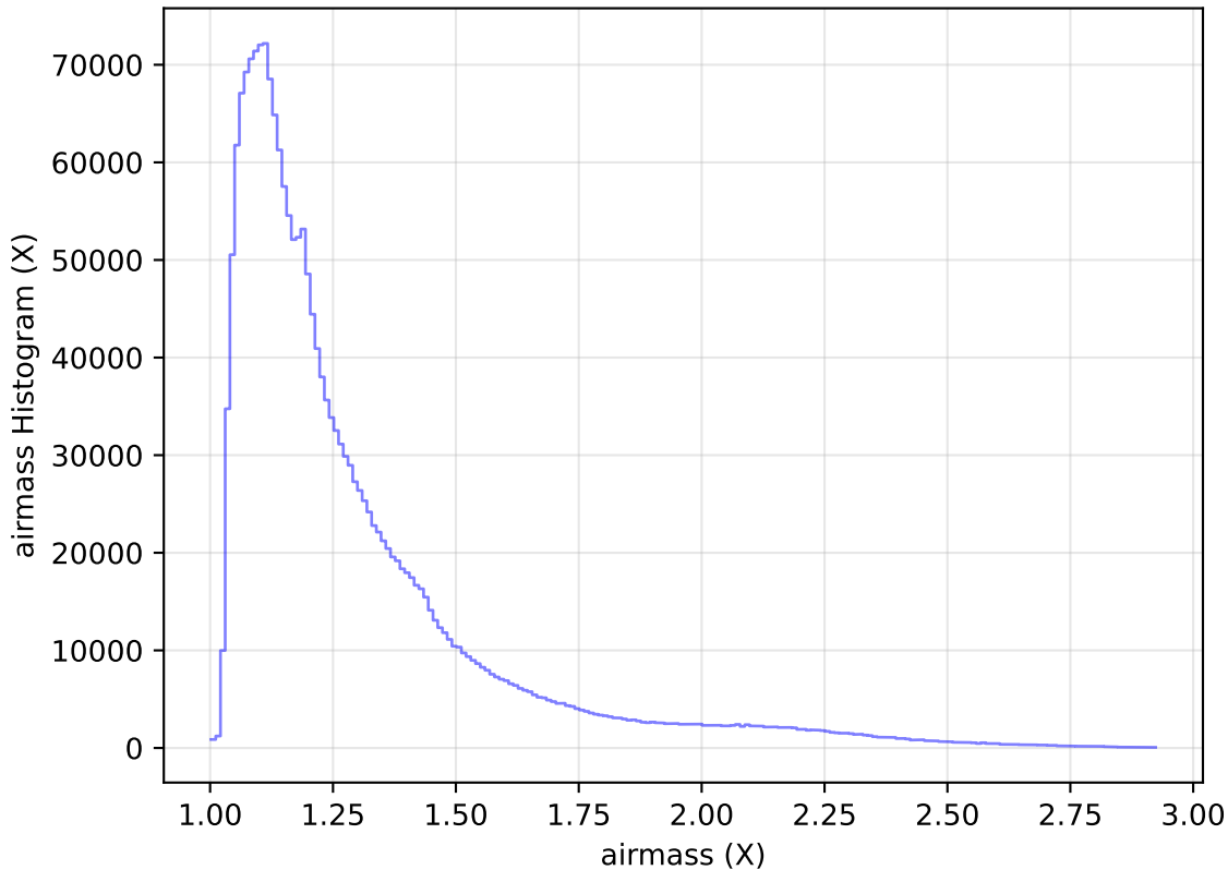
internal_u_expt27_nscale1.0v3.4_10yrs WFD all bands: airmass Histogram
