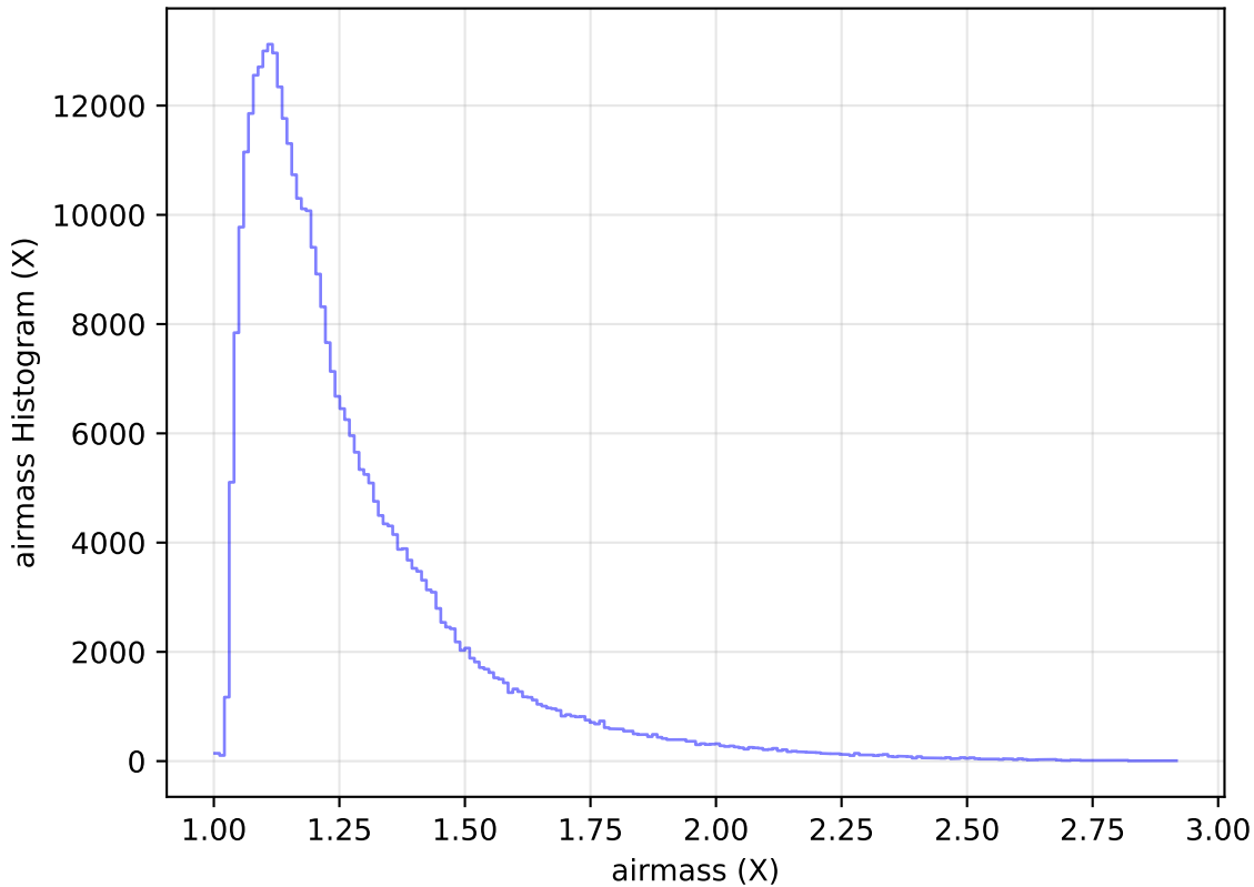
internal_u_expt27_nscale1.0v3.4_10yrs All sky y band: airmass Histogram
