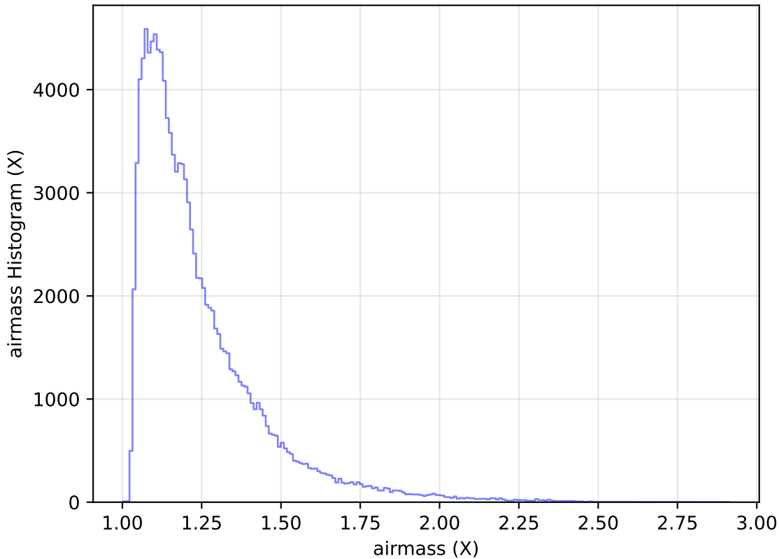
internal_u_expt27_nscale1.0v3.4_10yrs All sky u band: airmass Histogram
