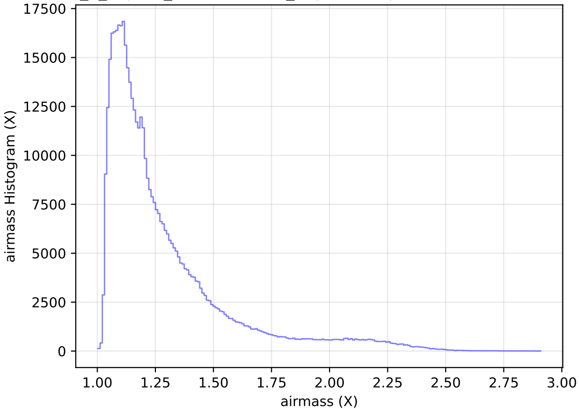
internal_u_expt27_nscale1.0v3.4_10yrs All sky r band: airmass Histogram
