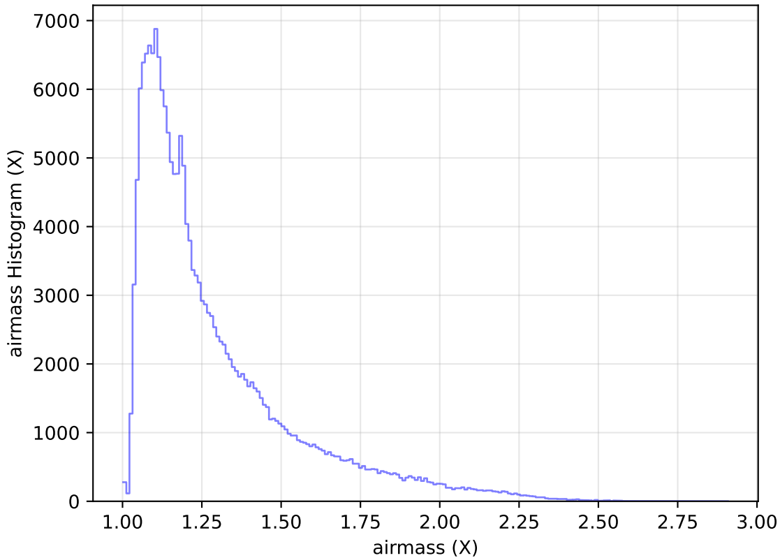
internal_u_expt27_nscale1.0v3.4_10yrs All sky g band: airmass Histogram
